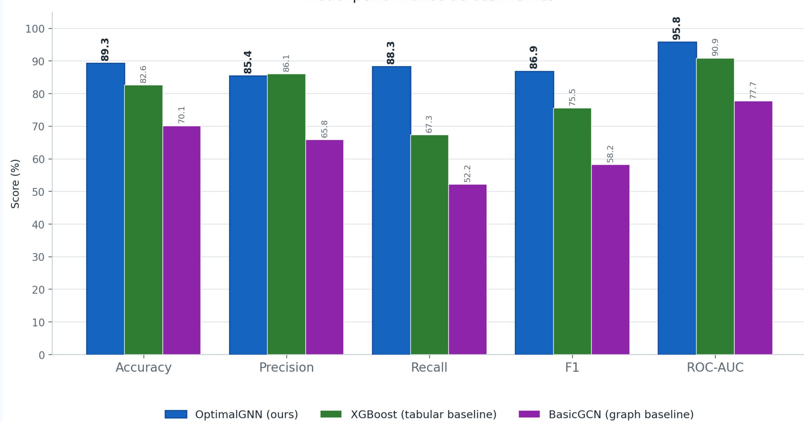
Model performance across metrics
